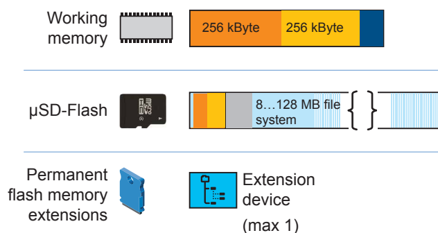
Memory structure of a PCD1.M2_ with additional memory cards
